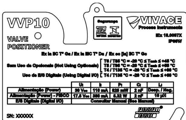
Figura 5.1 – Plaquea Ex ia do VVP10 PROFIBUS.
